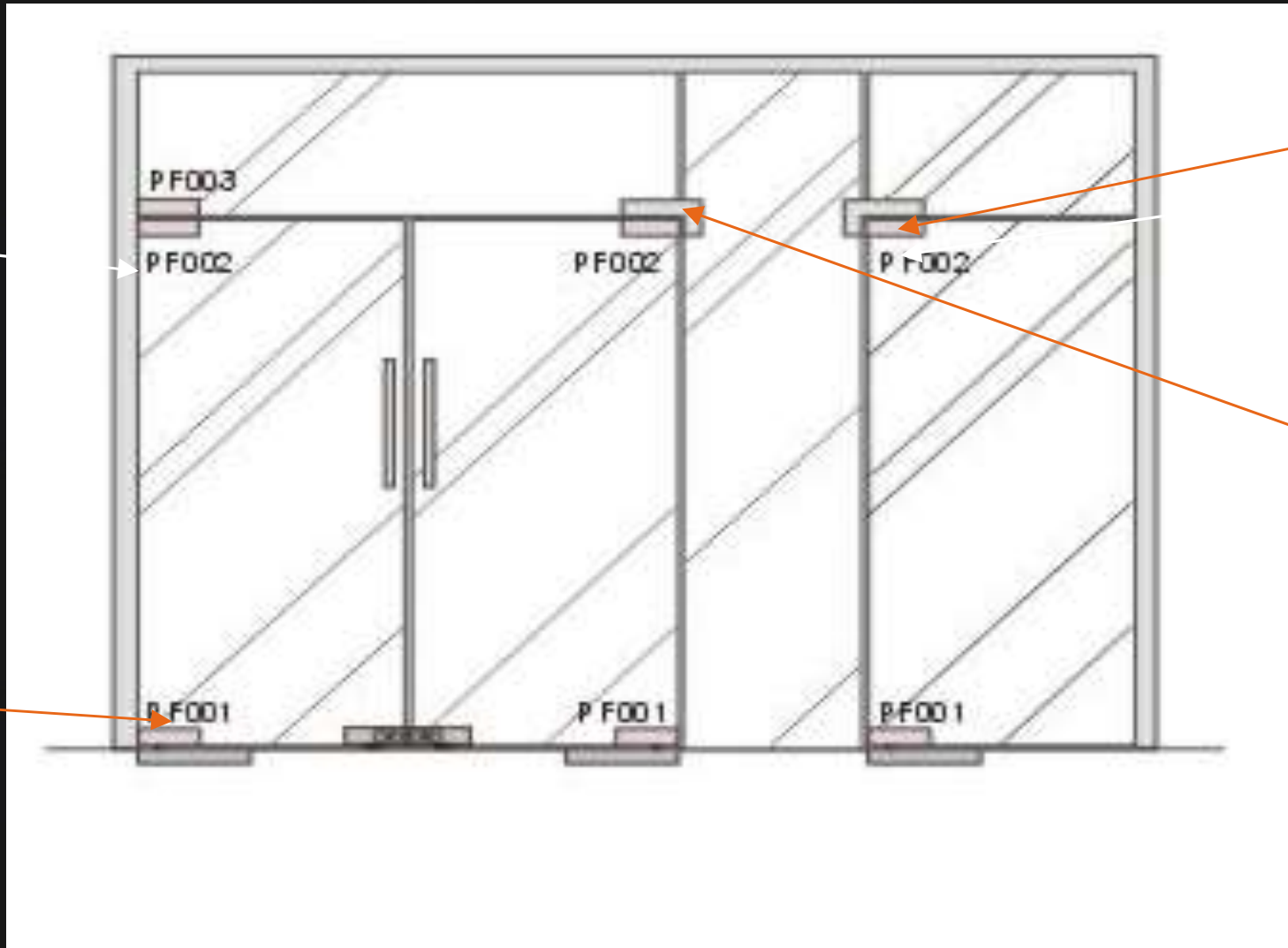
L-ARM WITH PIVOT
