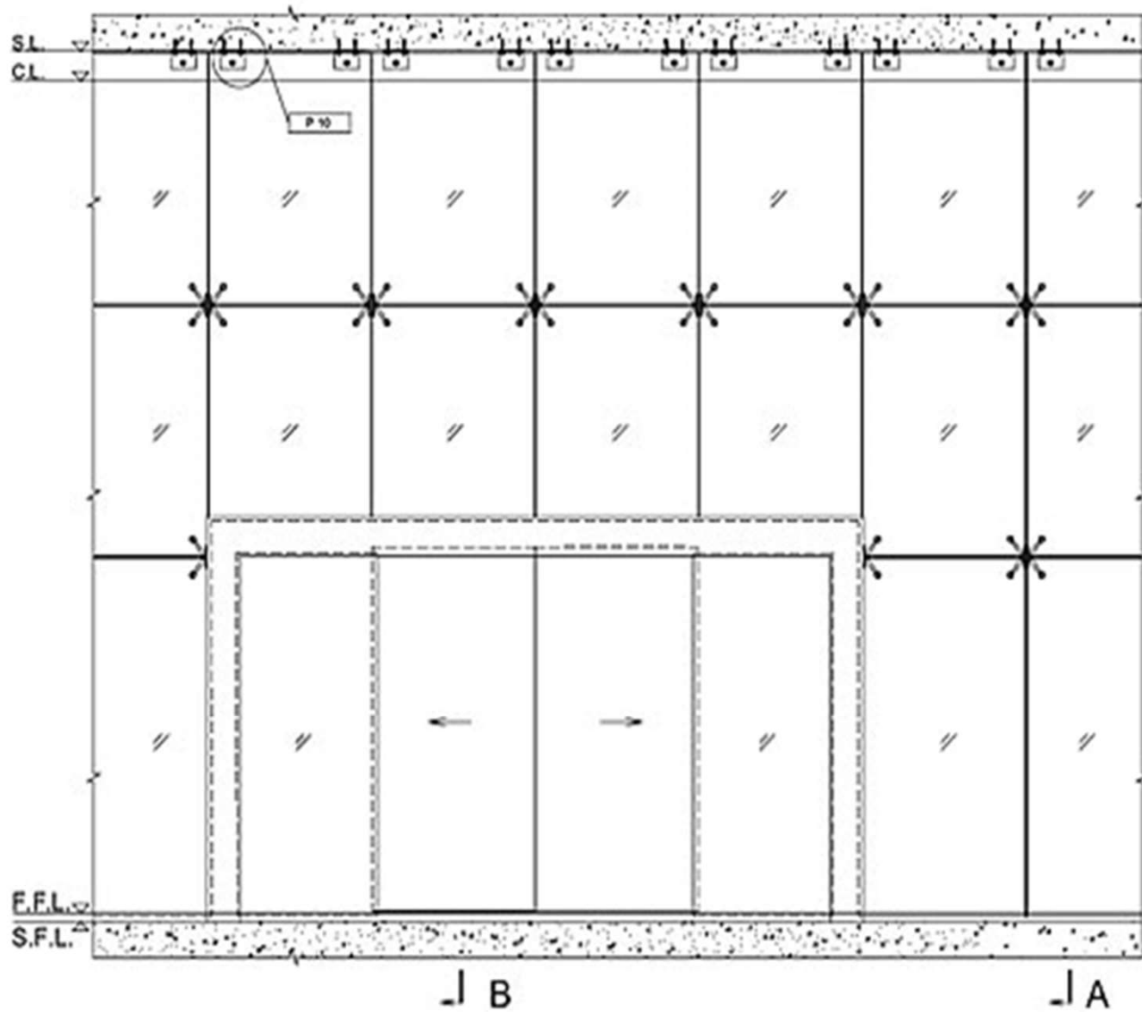
FRONT ELEVATION
