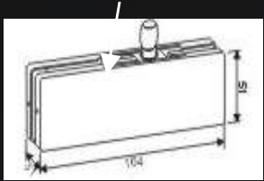
TOP PATCH WITH PIVOT
