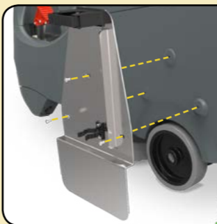
CRO Spray Mop Mounting Kit PN:903182
