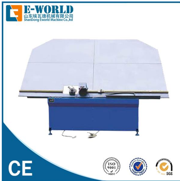
4.3 硅酮打胶机 silicone extruder machine
