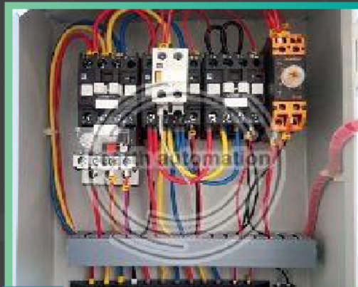
Star Delta Starter Control Panel
