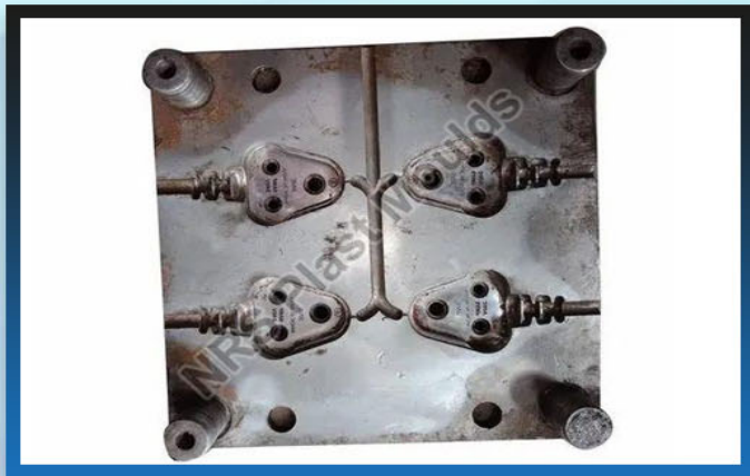
3 Pin Plastic Plug Injection Moulds
