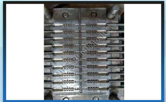
Plastic Electric Grip Injection Mold
