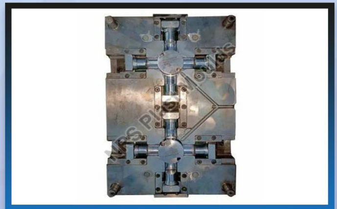
Plastic 4 Way Junction Box Injection Mold
