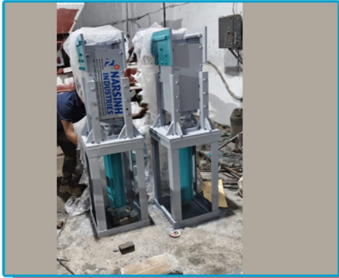
Interlocking Brick Making Machine
