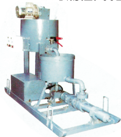
Grout pump
