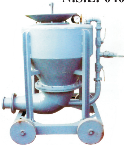
Concrete Placer
