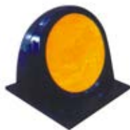
Model ID: SM-137 Dimension: Height: 105mm Bottom: 150 X 105mm Brand: 3M
