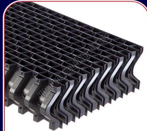
FRP Drift Eliminator
