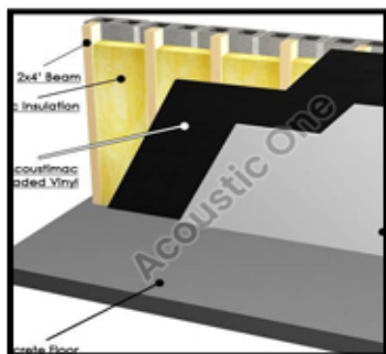
Sound Barrier Vinyl Sheets
