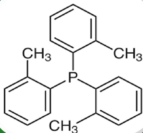
Tri-O-Tolyl Phosphine
