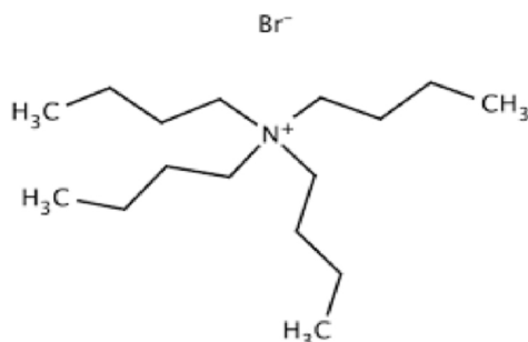
Tetra-n-butylammonium Bromide
