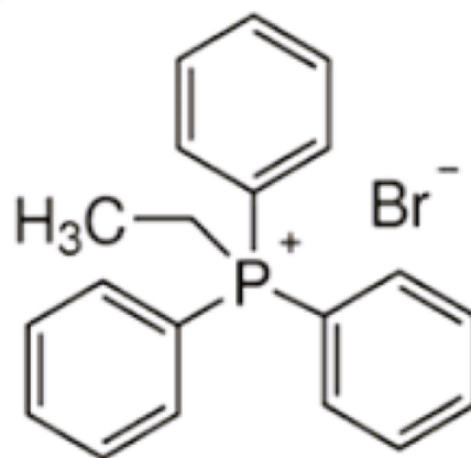
Ethyltriphenylphosphonium Bromide
