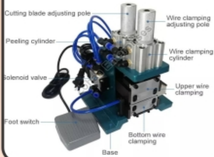
3F Semi Automatic Pneumatic Wire Stripping Machine
