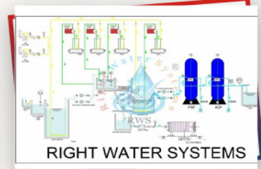
40 KLD Effluent Treatment Plant
