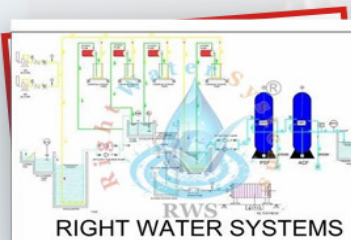
20 KLD Effluent Treatment Plant
