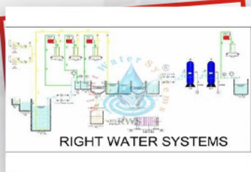
75 KLD Prefabricated Effluent Treatment Plant
