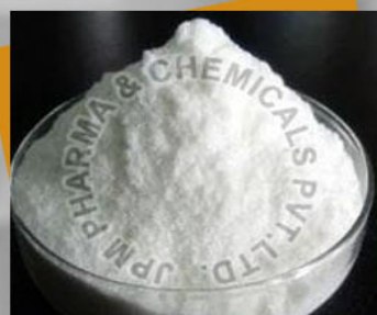
Butyric Acid
