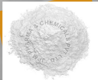
Cinnarizine
