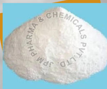
Butylated Hydroxytoluene
