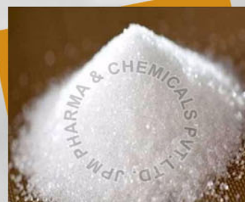
Citric Acid
