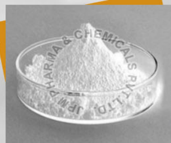
Benzoyl Chloride
