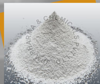
Calcium Chloride
