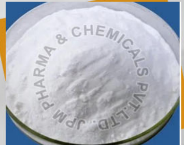
Dimethylamine
