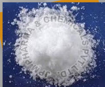
Carbon Tetrachloride
