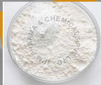
Albendazole
