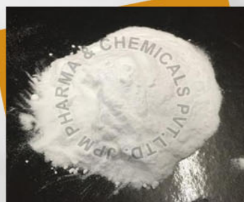
Boric Acid
