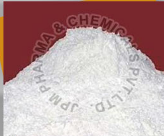
Chloramphenicol
