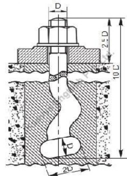
Bent foundation bolt
