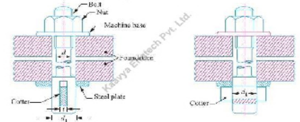
COTTER FOUNDATION BOLT
