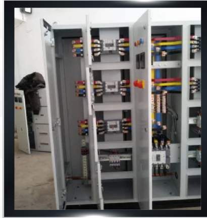
Double Busbar Panel
