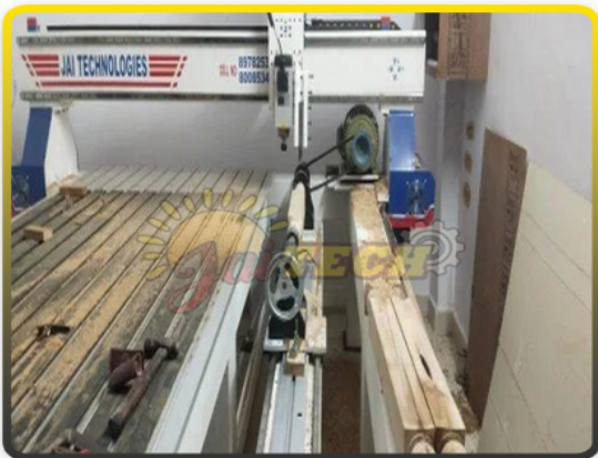
Turning CNC Wood Router Machine
