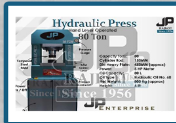
JP Gold Coin Die Pressing 80 Ton Hydraulic Press Machine
