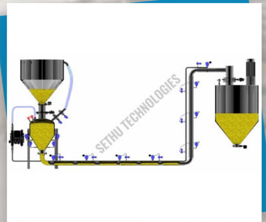
Pneumatic Conveying System
