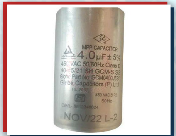
4 MFD 450 VAC Al Cane MPP Capacitor
