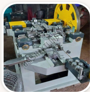
High Speed Wire Nail Making Machine
