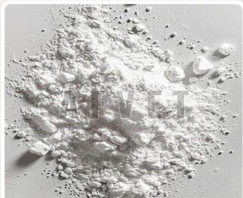
Mexoryl SX Terephthalylidene Dicamphor Sulfonic Acid
