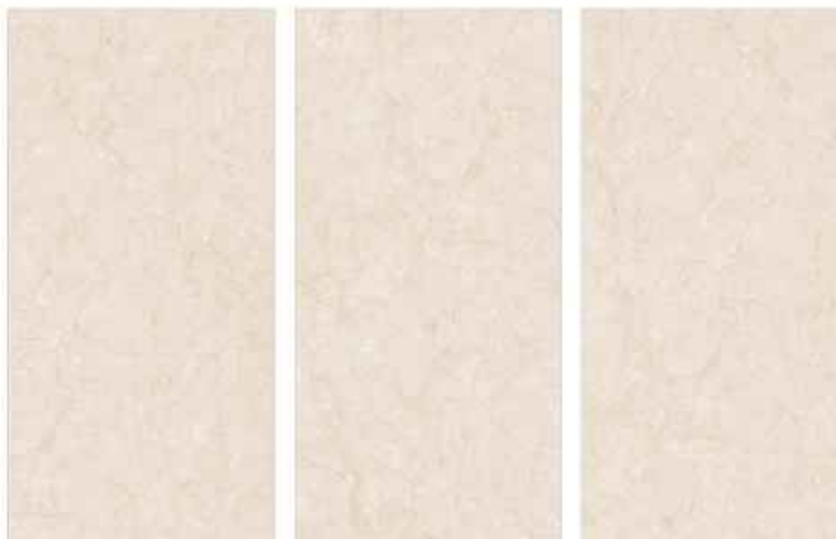
Random - 3 Faces
