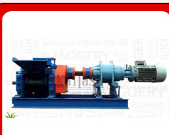
Super Jumbo Heavy Chottu Single Mill with Planetary Gear Box
