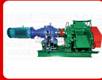
Super Deluxe-Single Mill with Planetary Gear Box
