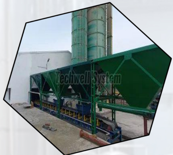
Fully Automatic Concrete Batching Plant
