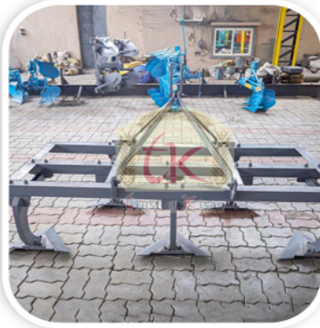
5 Tynes Duck Foot Tractor Cultivator
