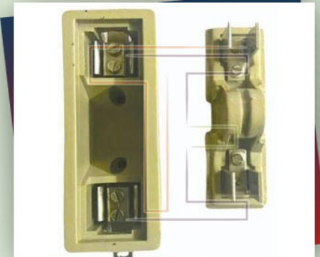
63A X 415V XL HANDLE KITKAT FUSE
