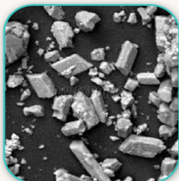
Lithium Aluminium Hydride
