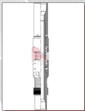
Spectramax RH Running Tool
