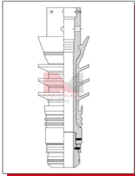
Spectramax Casing Wiper Plug
