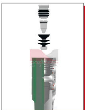
Spectramax MDV Mechanical Cementing Collar
