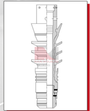
Spectramax Liner Wiper Plug
