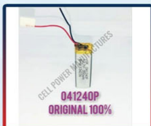
041240p 450mah originals lipo polymer battery
