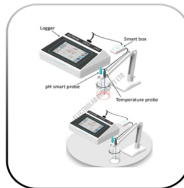
Digital PH Meter , For Laboratory
