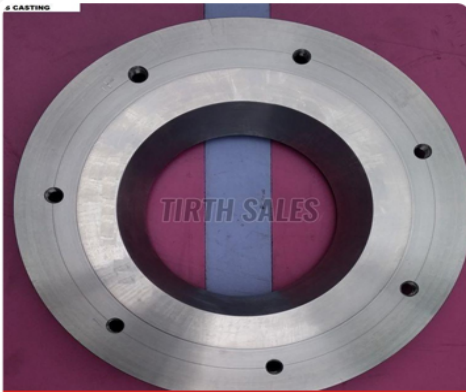
Polished Stainless Steel Investment Casting
