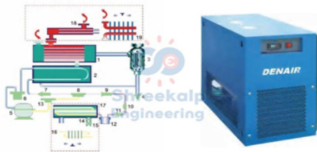
Refrigerated Compressed Air Dryer
