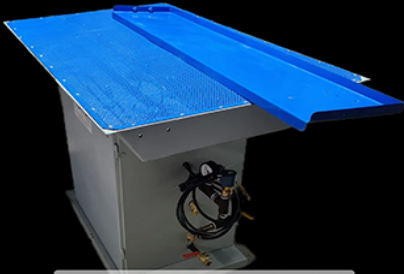
Inbuilt Steam vacuum table 6KW for garment use
