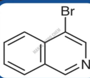
4-Bromoisoquinoline
