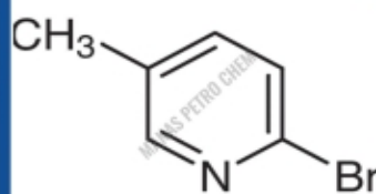
2-Bromo-5-methylpyridine
