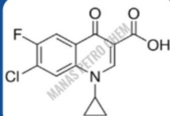
fluoroquino Ionic acid
