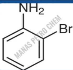
2-Bromoaniline CAS-615-36-1
