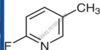
2-Fluoro-5-methylpyridine
