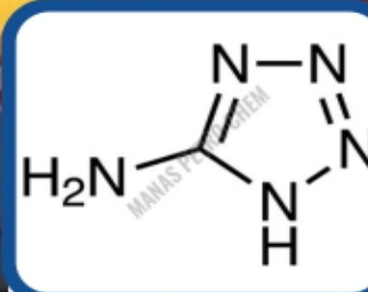
5-Amino-Tetrazole Anhydrous
