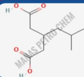
Isobutyl Glutaric Acid
