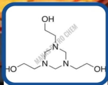
1,3,5 - Tris (2hydroxymethyl)hexa
