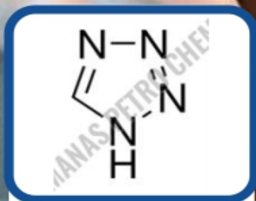
1 H Tetrazole CAS-288-94-8
