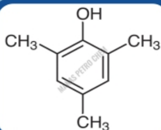
2,4,6-Trimethylphenol
