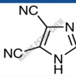
4,5-Dicyanimidazole
