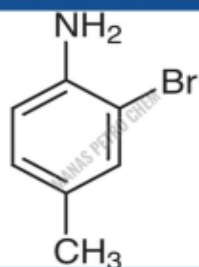
4-Bromo-2-methylaniline CAS
