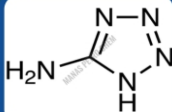
5 Amino Tetrazole Monohydrate
