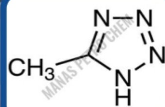
5-Methyltetrazole
