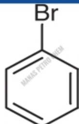
Bromobenzene
