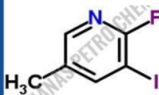
2-Fluoro-3-Iodo-5-Methylpyridine
