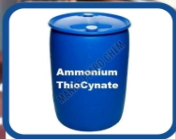
Ammonium Thiocyanate
