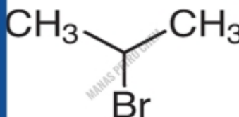
Iso Propyl Bromide (2- Bromo Propane)
