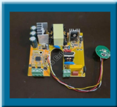
BLDC Ceiling Fan PCBA(Controller Board)
