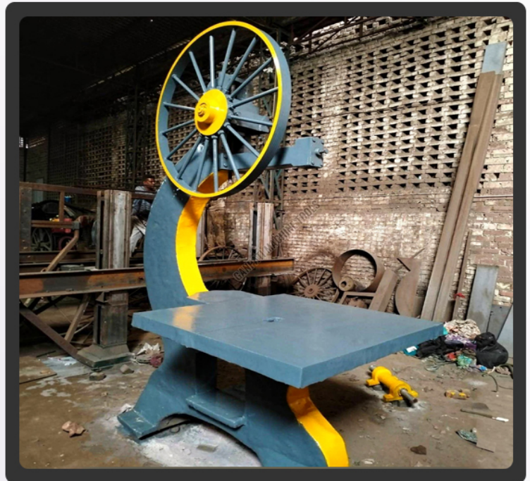
42 Inch Cast Iron Wood Cutting Bandsaw Machine
