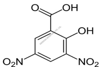
3,5-Dinitrosalicylic Acid
