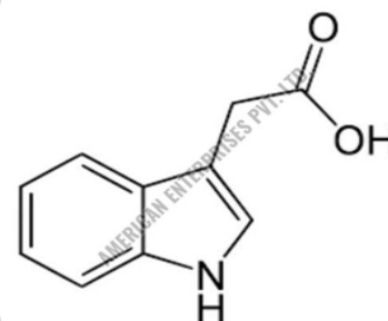
Indole-3-Acetic Acid
