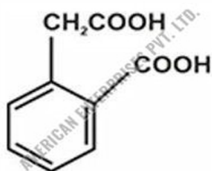
Homophthalic Acid
