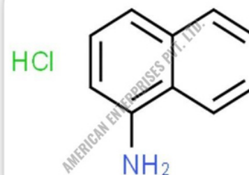
1-Naphthylamine Hydrochloride
