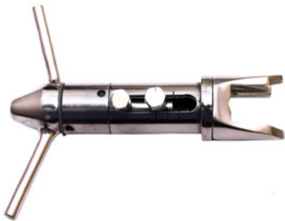
1410 Dynamic Wire Tenser Small
