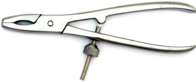
1239 Broken Head Screw Removal With Speed Lock Heavy Duty
