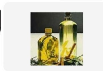
D-Carvone
