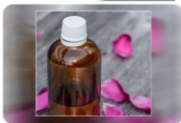
Terpinyl Acetate
