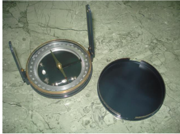
Survey Compass
