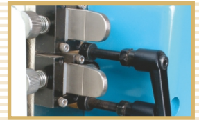
Gap setting adjustment by calipers
