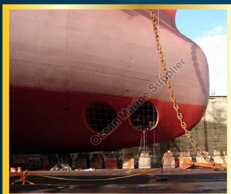
Bow Thruster
