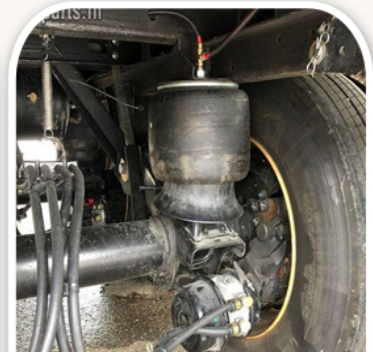
Utility Trailer Shock Absorber
