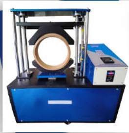
CORE COMPRESSION STRENGTH TESTER
