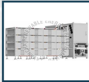
Deye SUN-100K-PCS01 HP3 C&I Energy Storage System
