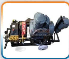
Flp High Pressure Hydro Test Pump
