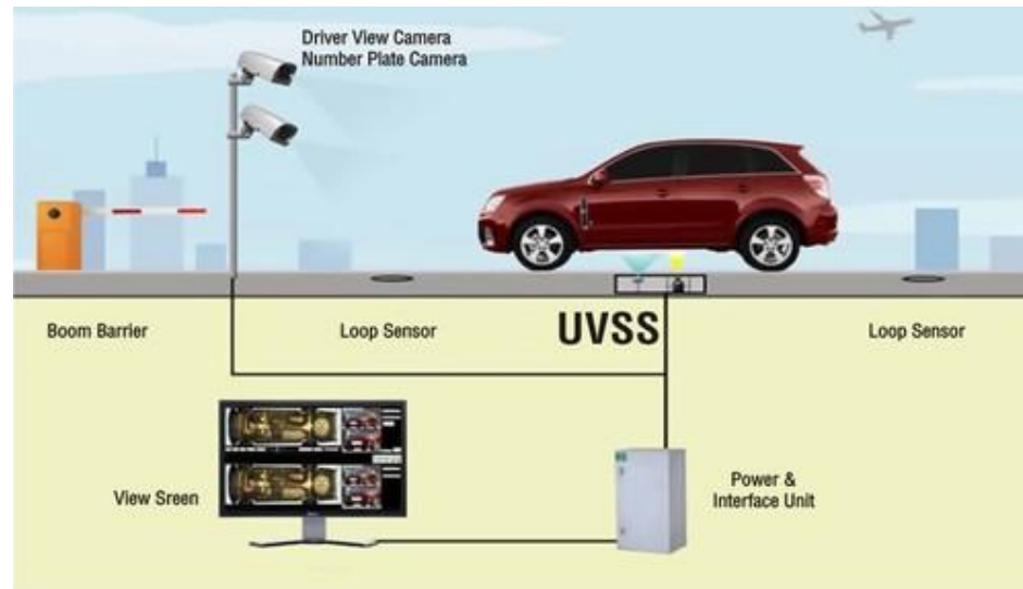
Under Vehicle Scanning System (UVSS)
