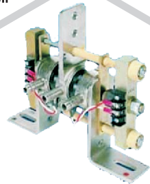
SCR Assembly
