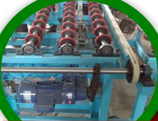
Roller Conveyor
